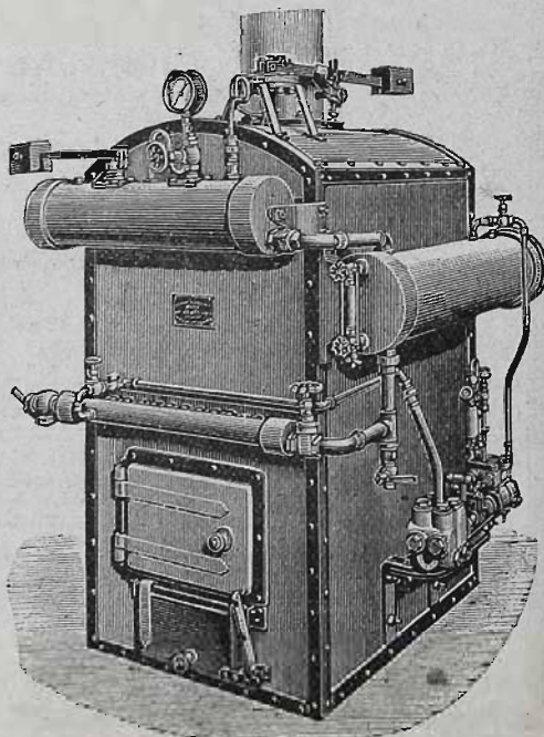
8 H.P. Boiler, fitted with Pump and Automatic Feed Attachment.
