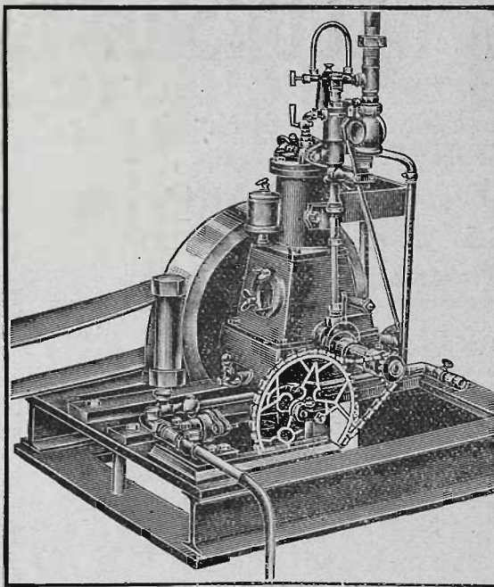
3 1/2 H.P. ENGINE.
