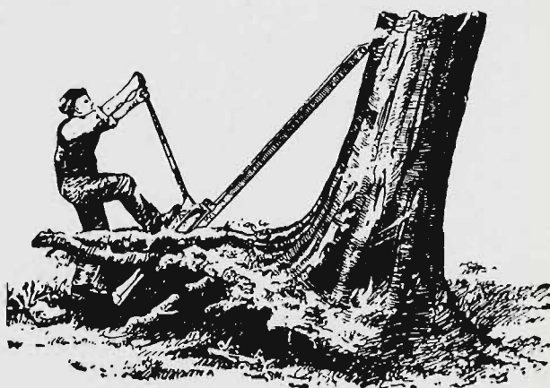
"MONKEY" JACK.
