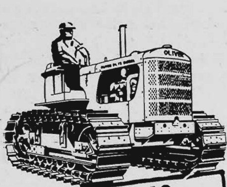
OC 12 6-cyl. Diesel 53.05 DBHP, 89 Belt HP
