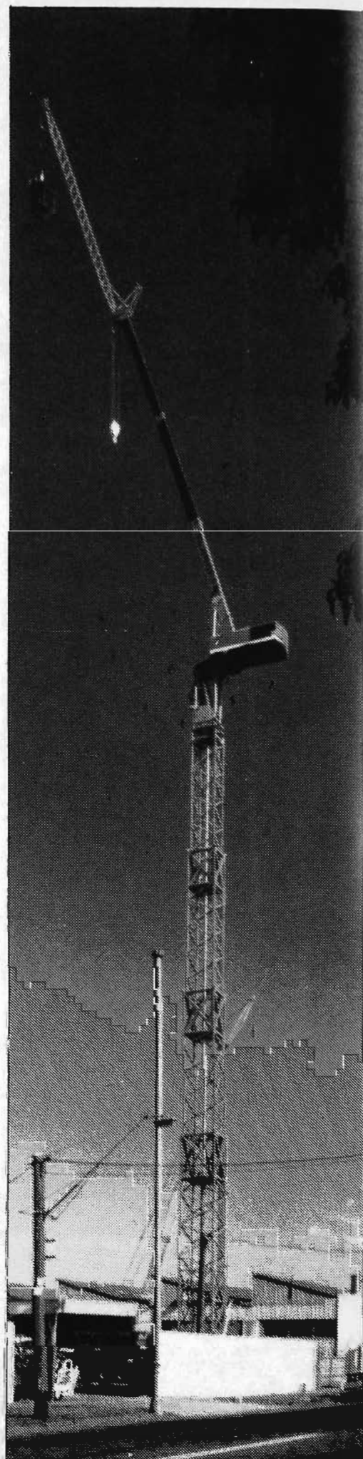
GCI5400 Maximum hook height 273 feet, reaches 217 feet in 16 minutes from folded position on arrival at site.
